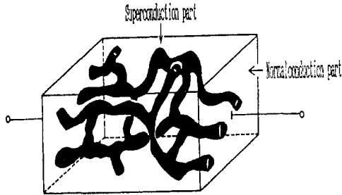
Fig. 1. The filament current path of superconducting bulk.
