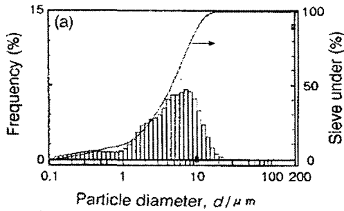
Fig. 1. Particle distribution of superconducting precursor.
