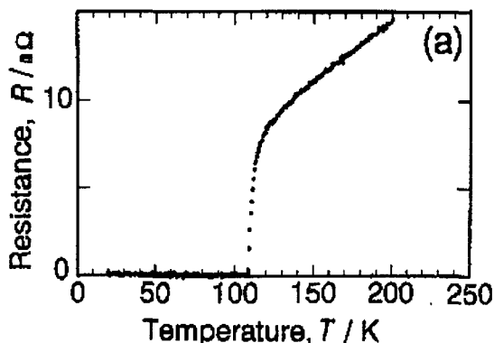
Fig. 3. Resistance-Temperature characteristics of superconducting precursor.
