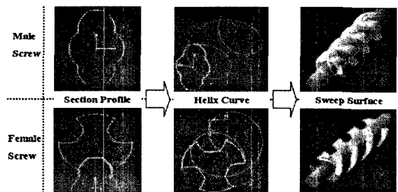
Fig. 3 Modeling process of screws
