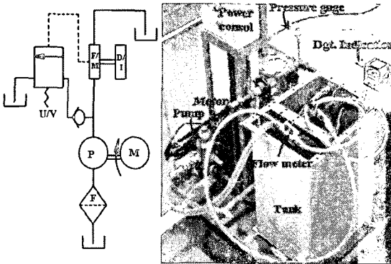
Fig. 12 Hydraulic circuit & performance test equipment
