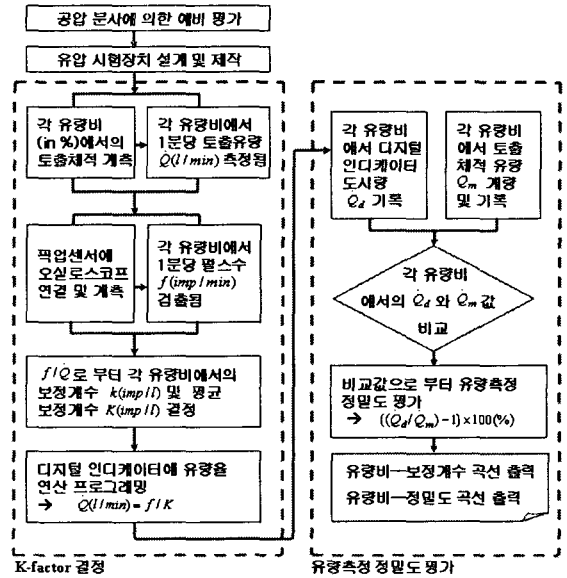
Fig. 10 Process of performance test
