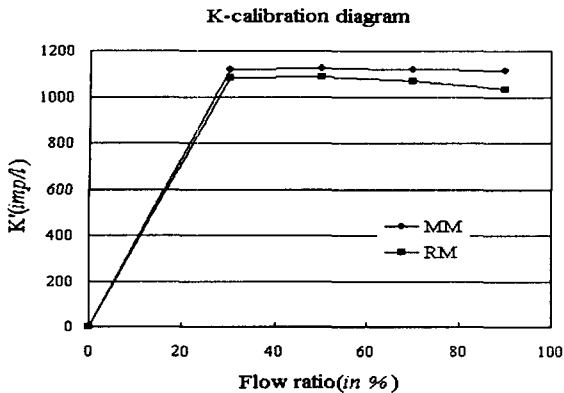
Fig. 13 K-calibration diagram
