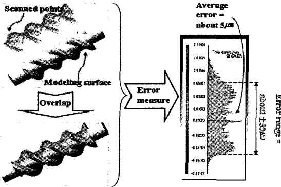
Fig. 4 Error analysis of reverse modeling
