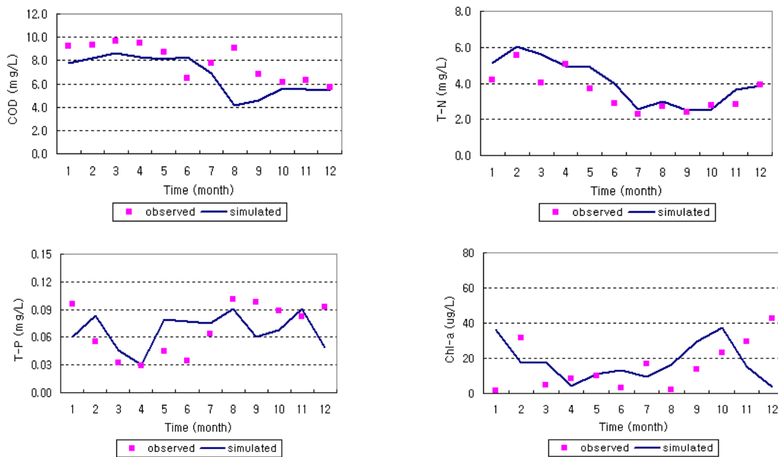
Fig. 3 Comparison of observed and simulated water quality for verification period
