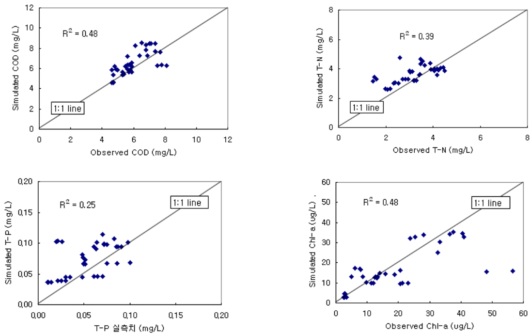
Fig. 2 Scatter diagram of water quality in the Geumgang lake for calibration period
