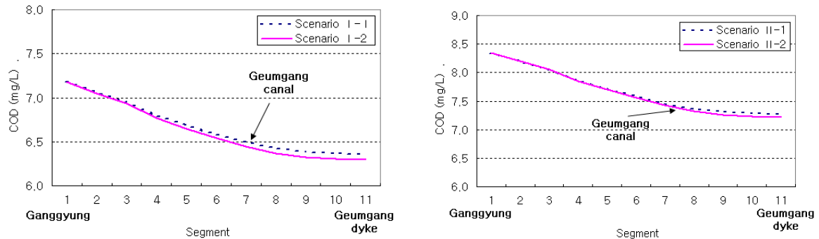
Fig. 4 Variations of COD concentration through Geumgang lake for each scenario
