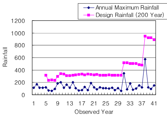
Fig. 4 Relation between design rainfall and observed year at Pohang station
