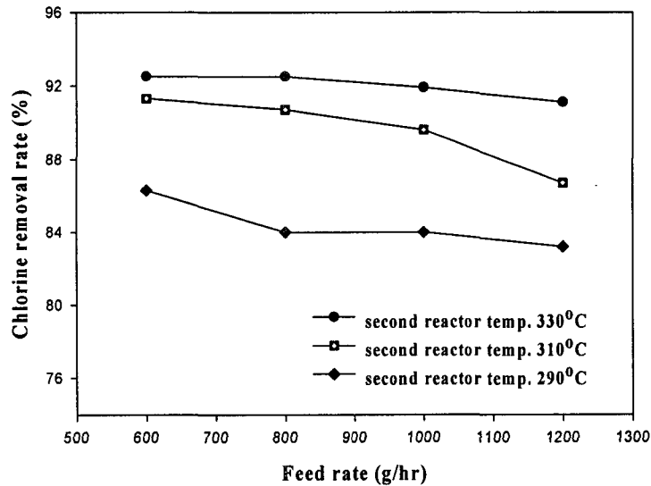
Fig. 6. Chlorine removal rate with feed rate and second screw reactor temperature.
