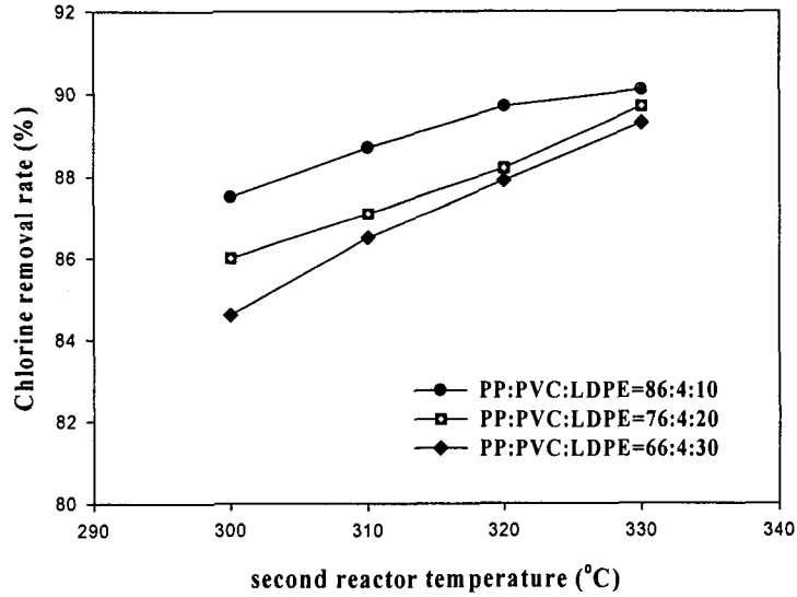
Fig. 5. Chlorine removal rate with second reactor temperature and viscosity.
