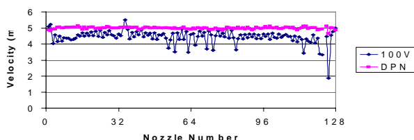
Fig 5. Drop Velocity Variation after DPN Correction
