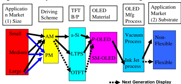
Fig.2 The Way of P-OLED Manufacturing
