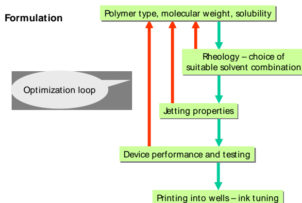
Fig 4. Optimum Ink Formulation Procedure.
