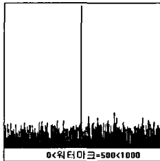
(e)워터마크=500
