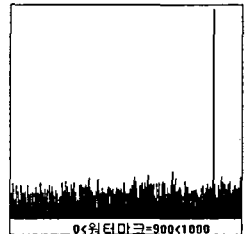
(f)워터마크=900
