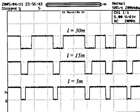
Fig. 5 Variations of control data due to line distance
