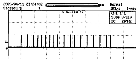
(a) PLC signal waveform
