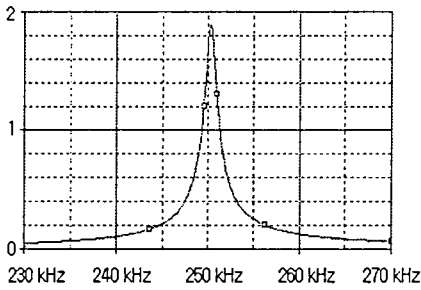
(c) PSpice simulation result Fig. 2 Coupling circuits and PSpice simulation result
