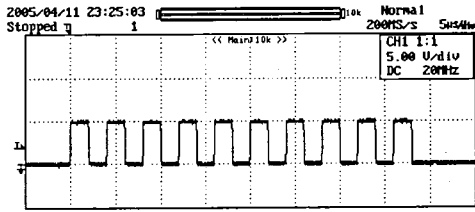
(b) Carrier waveform
