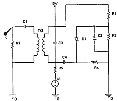
(a) Transmitter coupler
