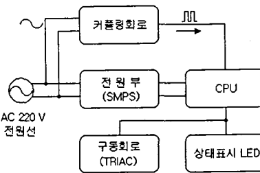
(b) Lamp receiver
