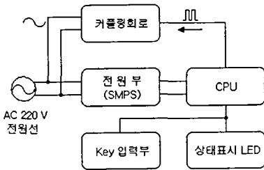
(a) Switch transmitter
