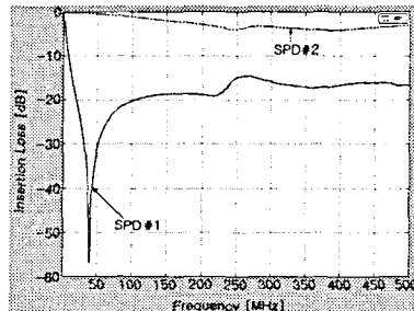
Fig. 3 Frequency characteristics of the SPDs
