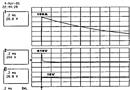
Fig. 6 Response waveforms to the 10/1000 \mu s surge current
