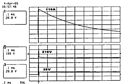
Fig. 5 Response waveforms to the 5/300 \mu s surge current
