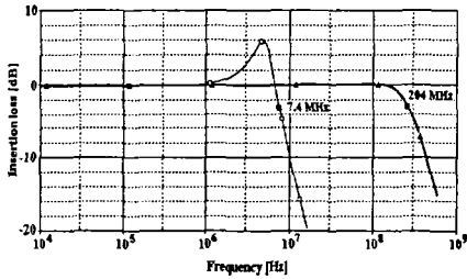
(a) Insertion loss
