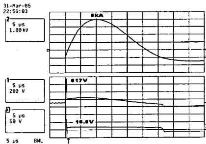
Fig. 4 Response waveforms to the 8/20 \mu s surge current
