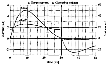
(b) Surge response
