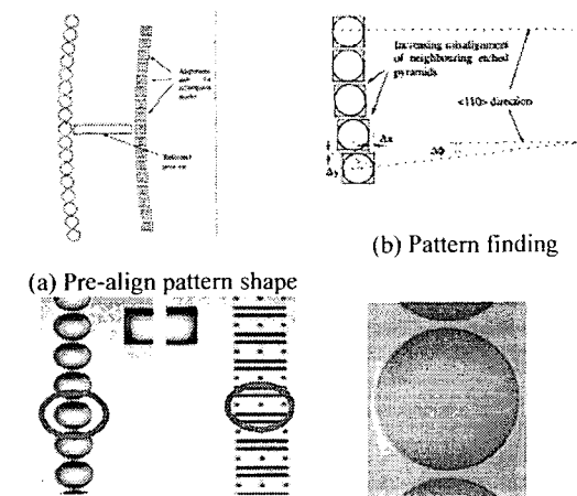
(a) Pre-align pattern shape (b) Pattern finding (c) Image of pattern after initial wet etching (d) Image after finding align pattern (x100)
