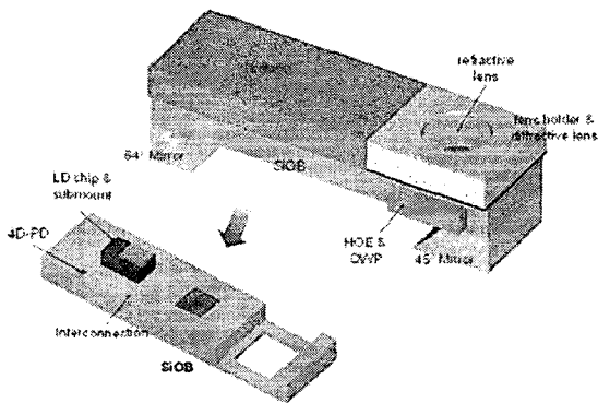
Fig. 1 Schematic view of integrated optical pickup
