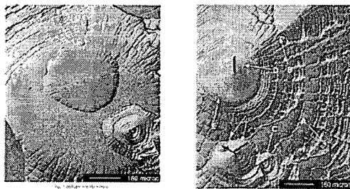
(a) Etch pits (b) Dislocation Fig. 4 Defects generated on (111) plane 8
