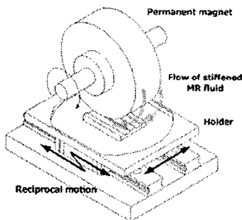
Fig. 6(a) Experimental setup
