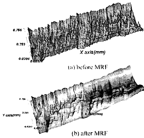
Fig.9 Topographical image of mirror plane before and after magnetorheological finishing
