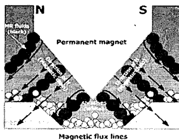
Fig. 6(b) Formation of magnetic chain
