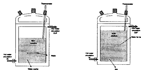
(a) horizontal loading (b) vertical loading Fig. 5 An apparatus for anisotropic etching
