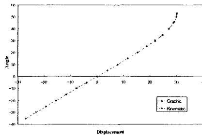
Fig. 4 Comparison between Graphical Analysis and Kinematic Analysis When the Link 2 is 30 mm
