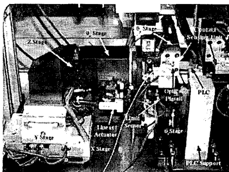
Fig. 6 Incident Channel Alignment Stage Assembly
