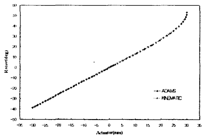
Fig. 5 Angular Displacement of Rotor for the Actuating Displacement in ADAMS Simulation
