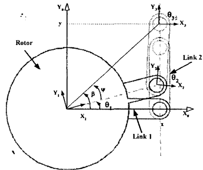
Fig. 3 Schematic Diagram for Kinematic Analysis
