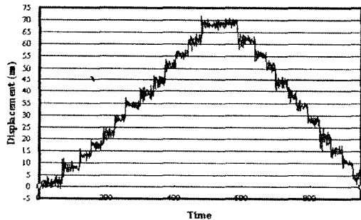
Fig. 3 Resolution of Ultra Precision Multi-Axis Stage
