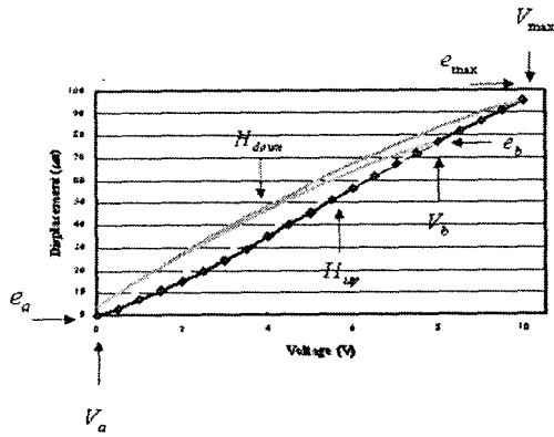
Fig. 5 Hysteresis Modeling
