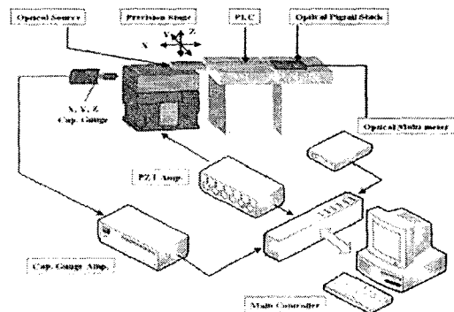
Fig. 2 Schematic Diagram of Ultra-Precision Optical Alignment System
