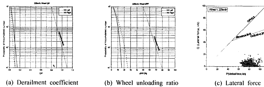
Fig. 3 Calculation results for KTX (1/40, 225km/h)
