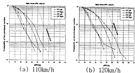
Fig. 8 Wheel unloading Ratio in curves (600R)
