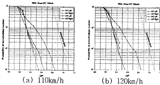
Fig. 7 Derailment coefficient in curves (600R)
