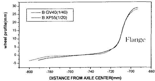
Fig. 2 Wheel profile of GV40 and XP55
