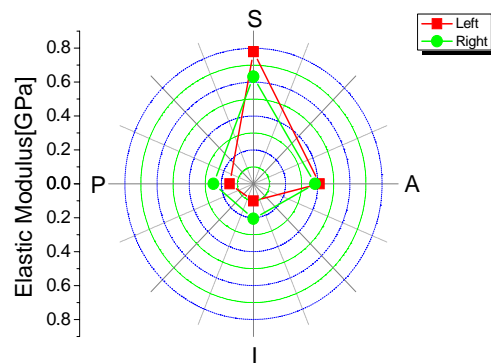
Fig. 6 Elastic modulus of femoral neck-2
