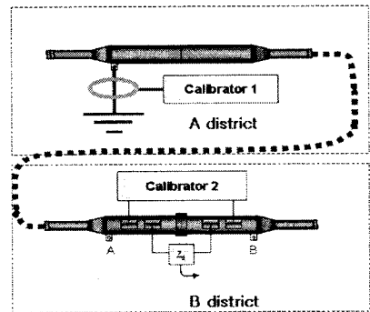
Fig. 1 Calibration test
