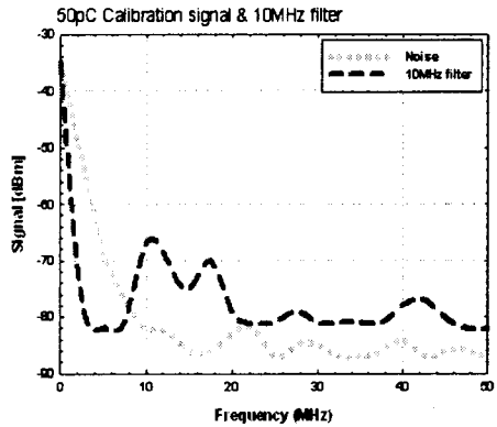
(b) Calibration signal injected in NJB
