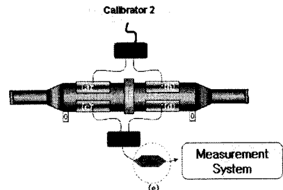
Fig. 2 The foil electrode sensor detection method that applied a filter
