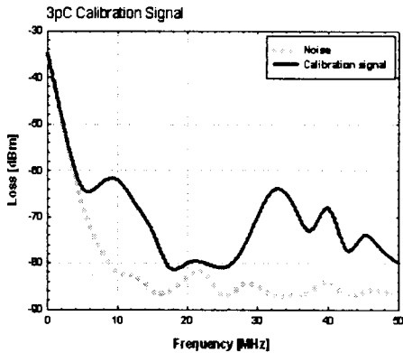
(a) Calibration signal by using the CT sensor at IJB
