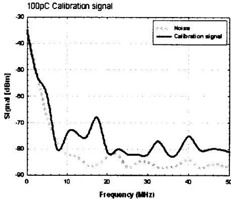
(b) Calibration signal by using the HFCT at NJB
