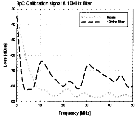
(a) Calibration signal injected in IJB
