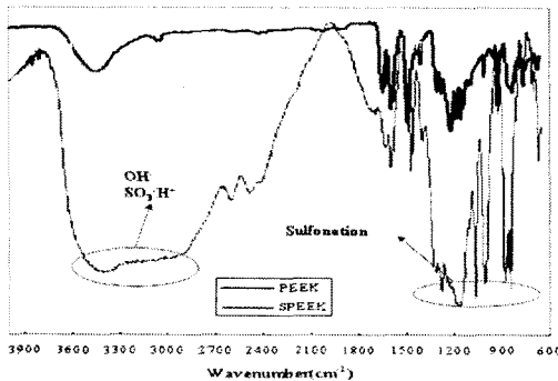
Fig. 2. FT-IR of PEEK & SPEEK
