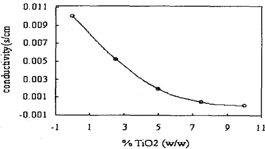
Fig.5. Proton conductivity of PVdF/SPEEK composite membranes as a function of the TiO 2 weight percentage.
