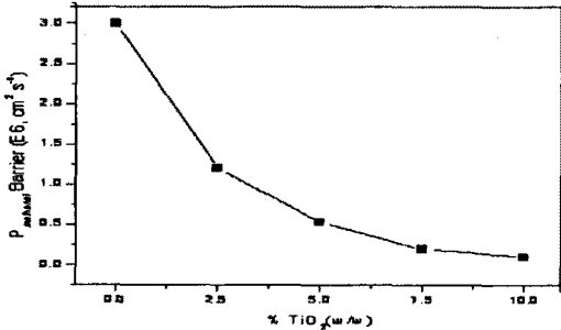
Fig. 4. Methanol permeability of PVdF/SPEEK composite membranes as a function of the TiO 2 weight percentage
