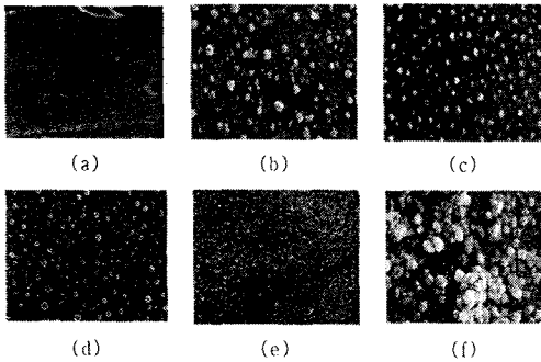
Fig. 1. Scanning electron micrograph of PVdF/SPEEK/TiO 2 composite membrane. (a)0.0% TiO 2 , (b)2.5%,(c)5.0%, (d)7.5%, (e)10.0%,(f)12.5%
