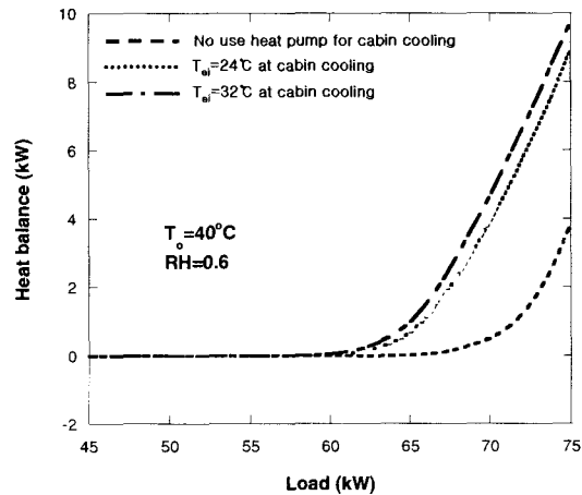
Fig. 3 Heat balance(=amount of stack heat release-radiator capacity) with respect to the load of a vehicle
