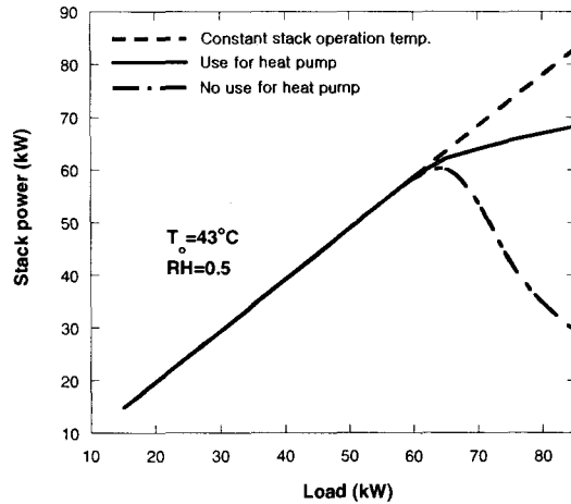
Fig. 4 Stack power with respect to the load of a vehicle
