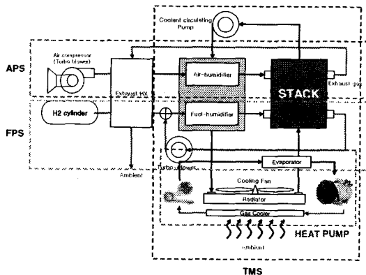
Fig. 1 Schematic diagram of a PEMFC system
