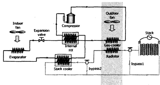
Fig. 2 Design of a heat release system
