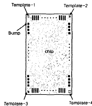
Fig. 1 The four templates and bumps on chip
