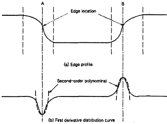
Fig. 4 Edge profile and first derivative distribution curve
