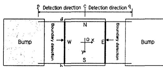
Fig. 2 Boundary detection to +x and -x direction from bump center point
