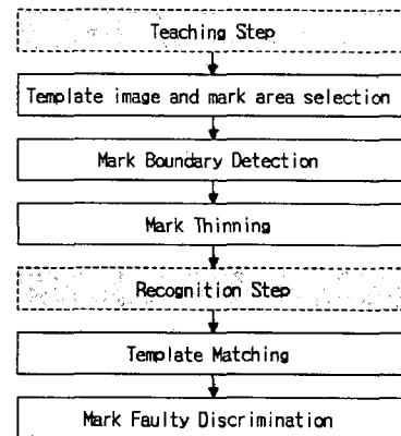
Fig. 1 Mark inspection system flowchart
