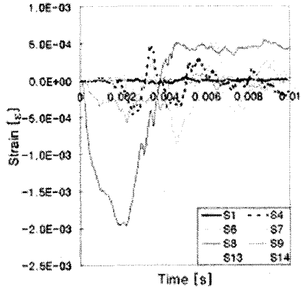
(b) 300 Hz Lowpass Filtering 변형률
