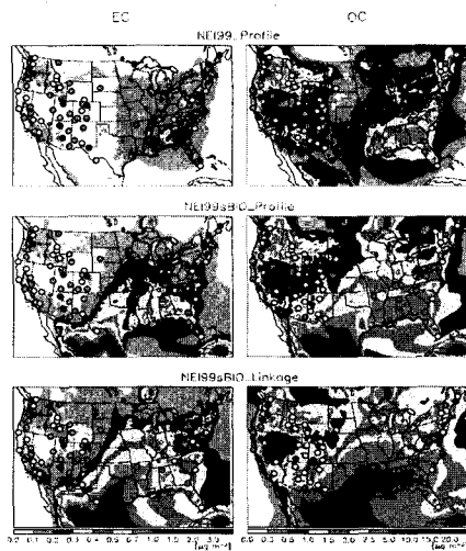
Fig. 1. Simulated monthly mean spatial distribution of EC/OC concentration in the lowest bottom layer of model ( \sigma value=0.998) under three run scenarios.
