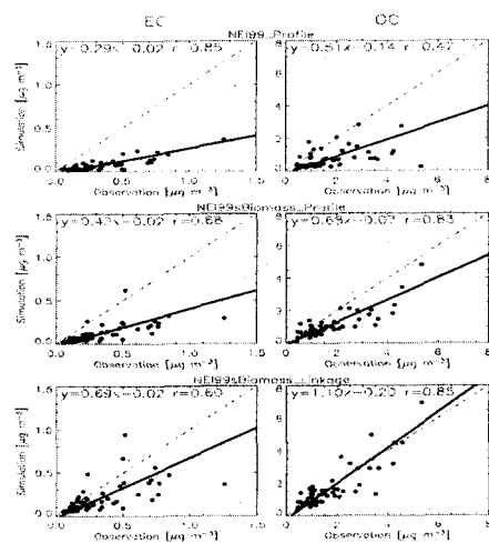
Fig. 2. Scatter plots of EC/OC monthly mean simulated versus observed values at IMPROVE sites under three run scenarios.
