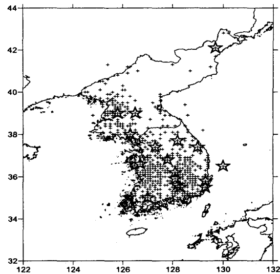
Figure 1. The distribution of historical earthquakes. The earthquakes are represented as '+', and large earthquakes used in this study are represented as pentagrams.
