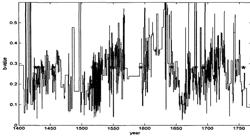
Figure 5. The variation of b-values(blue line) calculated from earthquakes in preceding 13 years and in 1.1° by 1.1° square about the each historical earthquakes with the distribution of large earthquakes(red asterisks).
