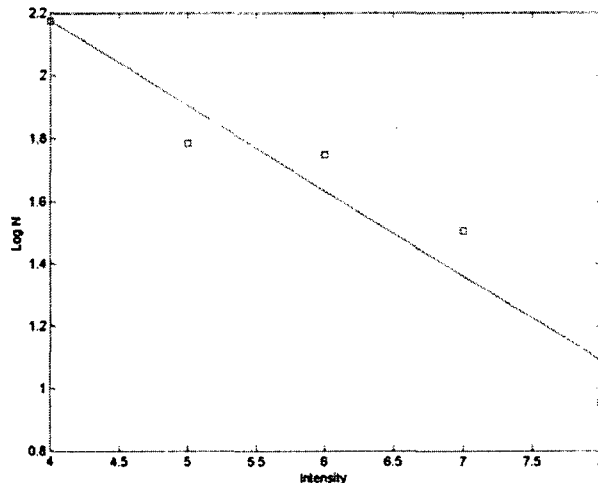
Figure 4. Linear regression of the distribution of intensity and logarithmic frequency of the whole foreshocks of 11 large earthquakes, \text{Log } N = 3.26 - 0.27 I_0 .
