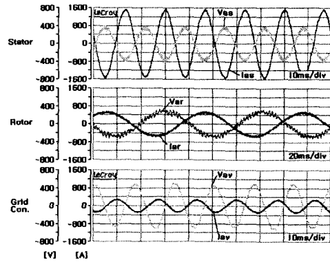
Fig.11 power factor control characteristics under the 1.2MW generation condition (@1440rpm)
