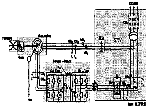
Fig. 1 The tidal power plant with a DFIG and electrical energy converter
