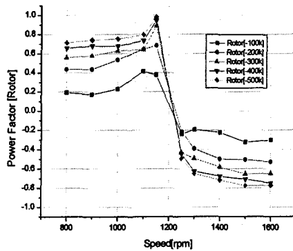
Fig. 7 Power factor characteristics at the rotor side converter
