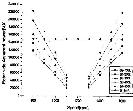
Fig. 9 apparent power characteristics according to stator power magnitude
