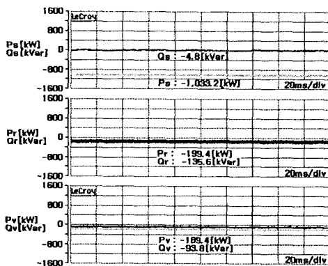
Fig. 10 power control characteristics under the 1.2MW generation condition (@1440rpm)
