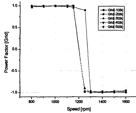
Fig. 6 Power factor characteristics at the grid side converter
