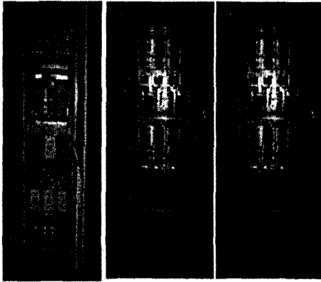
Fig. 2 Prototype of an electrical converter for doubly-fed induction generator
