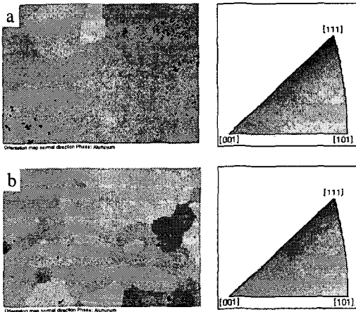
Fig.2.Orientation map normal direction. (a) Initial sample, (b) 4 passes ECAPed and annealed at 400 ° C/1 hour.
