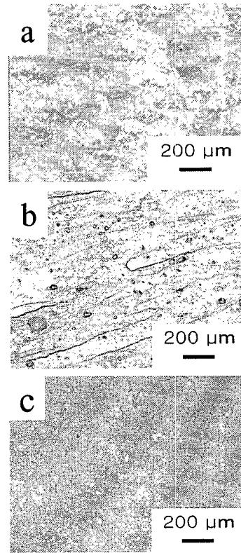
Fig.1. Optical micrographs obtained from the side surfaces of Al sheet; (a) initial Al sheet, and (b) 1 passes, (c) 4 passes and heat treated at 400°C / 1 hour.
