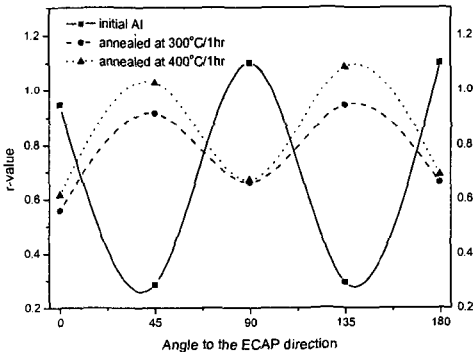
Fig.3. The variation of measured r-value as a function of ECAP direction for the initial Al sheet, and the 4 passes ECAPed and subsequent annealed Al sheets.
