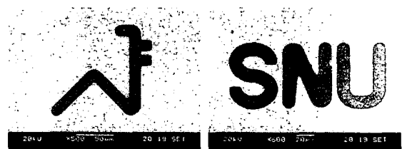
Fig. 5 Curved holes punched on titanium foil, emblem of SNU and letters 'SNU' with 14 \mu m in width
