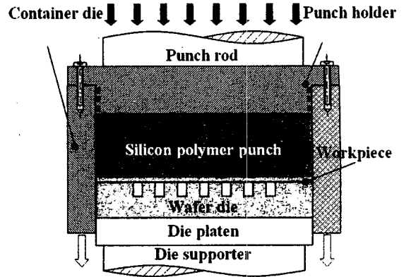
Fig. 1 Schematic of flexible punching process
