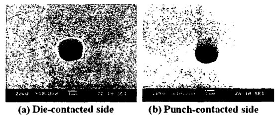
Fig. 3 Punched hole of copper foil ( d=2.3\mu m )
