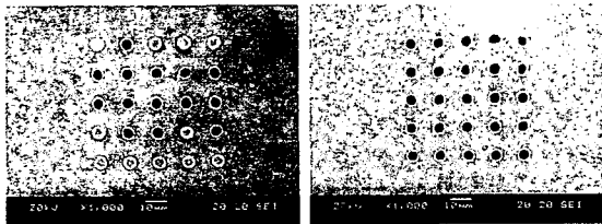
(a) As rolled foil (b) As annealed foil Fig. 6 Punching result of as rolled and as annealed foil
