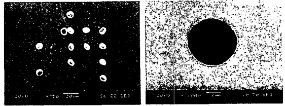
(a) Punched holes with dry etched die
