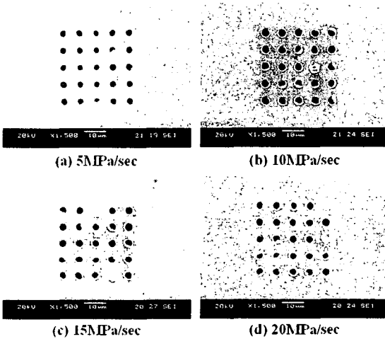
Fig. 9 3 \mu m-diameter holes punched on copper foil at 1.6GPa
