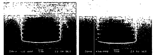
(e) As dry etched Si wafer (f) Die, after wet isotropic etching
