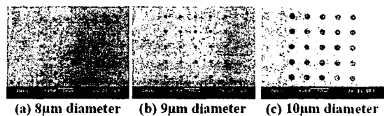
Fig. 4 Punched hole array of titanium
