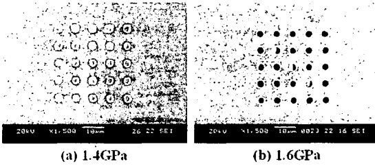
Fig. 8 3 \mu m-diameter holes punched on copper foil at 2MPa/sec
