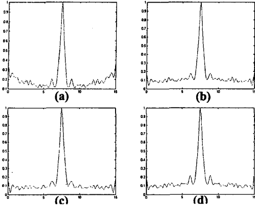
Fig. 6 Normalized line integrated intensity profile at Talbot position of (a) MLA without aperture array, (b)MLIAA with 5µm aperture, (c)MLIAA with 10µm aperture, and (d)MLA with dark corner
