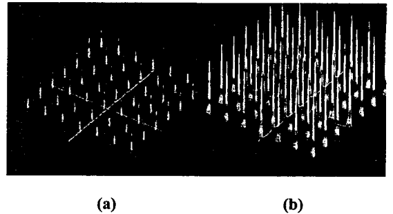
Fig. 11 Intensity profile of optical probes at Talbot position by (a)aperture array without MLA and (b) MLIAA with 10 \mu\text{m} diameter
