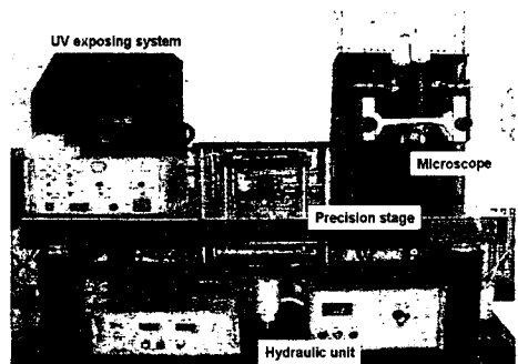
Fig. 8 Picture of monolithic lithography integration system
