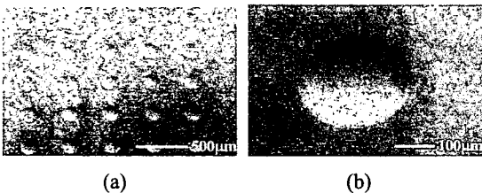
Fig. 5 SEM images of the fabricated nickel mold insert for (a) 200\mu\text{m} -diameter microlens array and (b) 300\mu\text{m} -diameter microlens.
