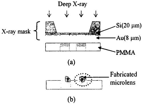
Fig. 1 Proposed microlens fabrication process: (a) Step 1: x-ray irradiation and (b) Step 2: thermal treatment [7,8].
