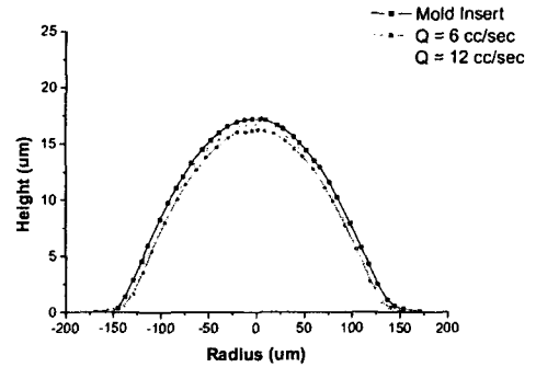
Fig. 8 Surface profiles of 300µm-diameter microlenses of the mold insert and injection molded PMMA substrates at different injection flow rates of 6 and 12cc/s.
