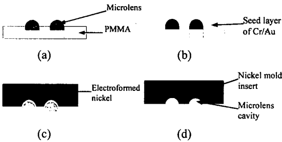
Fig. 4 Fabrication process of microlens mold insert: (a) microlens arrays on a PMMA sheet by the modified LIGA process, (b) seed layer deposition, (c) nickel electroforming and (d) nickel mold insert.
