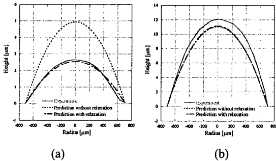
Fig. 3 Predicted microlens shapes ( 1500\mu\text{m} in diameter) in comparison with experimental ones (solid curve) at heating temperature of (a) 105^\circ\text{C} (b) 115^\circ\text{C} .
