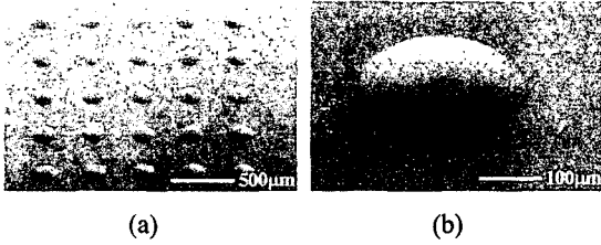
Fig. 7 SEM images of embossed PMMA: (a) 200µm-diameter microlens array and (b) 300µm-diameter microlens.
