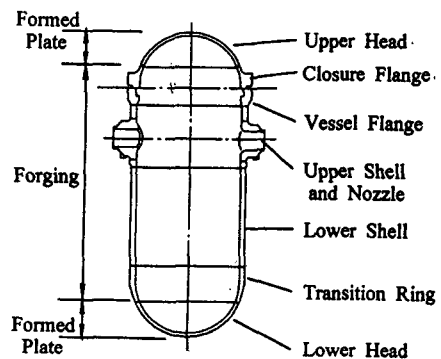
Fig. 1 Reactor vessel of 1,000MW nuclear power plant
