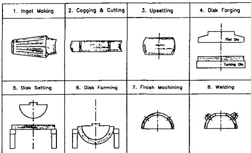
Fig. 2 Typical manufacturing process of head for 1,000MW nuclear power plant
