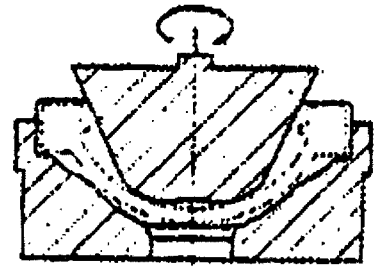
Fig. 5 Forging concept of JSW (3)
