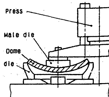
Fig. 3 Outside head forming apparatus (2)
