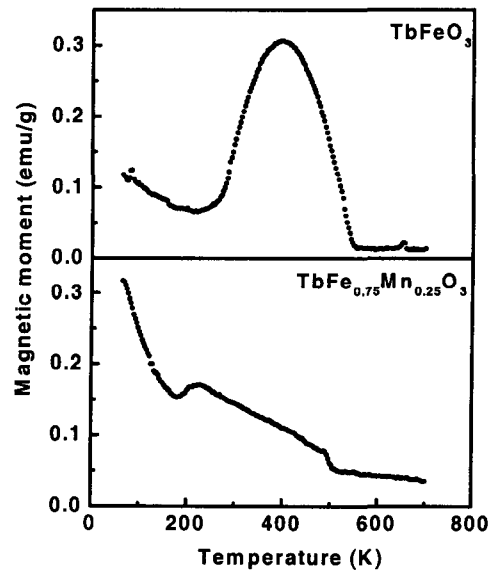
Fig. 2. Temperature dependence of the magnetic moment under an applied field of 200 Oe for TbFeO_3 and TbFe_{0.75}Mn_{0.25}O_3 .
