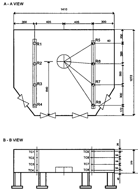
Fig.2 Schematic Diagram of the Test Section
