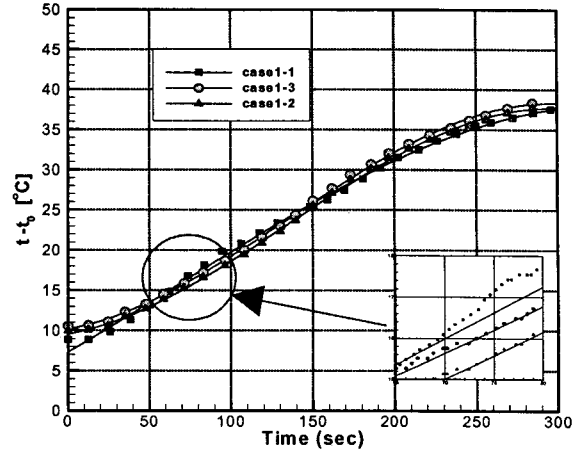
Fig. 10 Comparison of temperature distribution of TC15 at case 1
