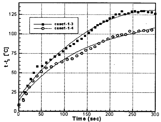
Fig. 12 Comparison of center fire temperature distribution of TC9 and TC13 at case 1
