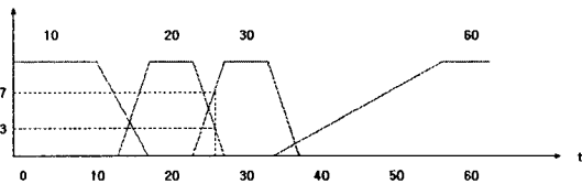
Fig. 12 Linguistic label expression of TG data
