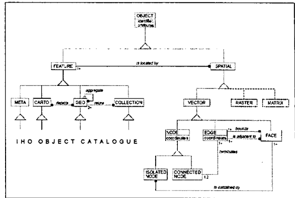
Fig. 1 Object Structure of S-57
