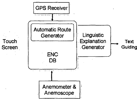
Fig. 4 Block diagram of VOSS
