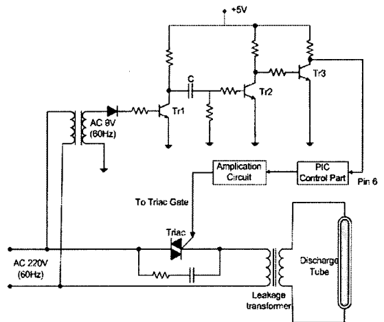
Fig. 1 The electrical circuit consisting of three major components : a ZCS circuit, a PIC one-chip microprocessor, and a discharge circuit.
