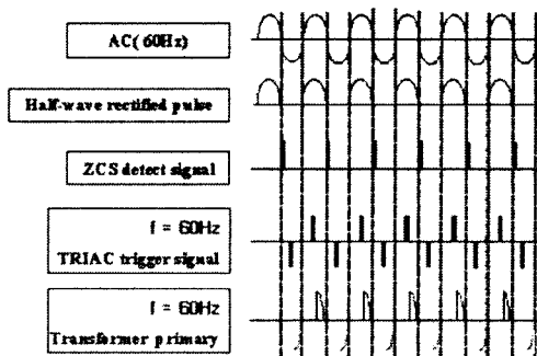
Fig. 2 The voltage waveform of the AC line, pulse signals generated from the ZCS circuit, and the gate trigger signals with trigger pulse delay angle of 90 at 60Hz.
