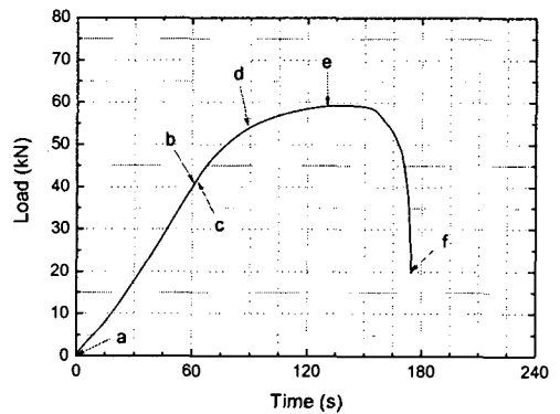
Load vs. time
