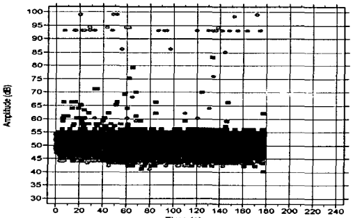
Amplitude vs. time (b) notched type
