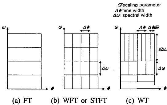
Fig. 1 The corresponding resolution on the time-frequency plane
