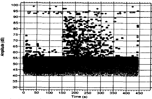
Amplitude vs. time (a) smooth type
