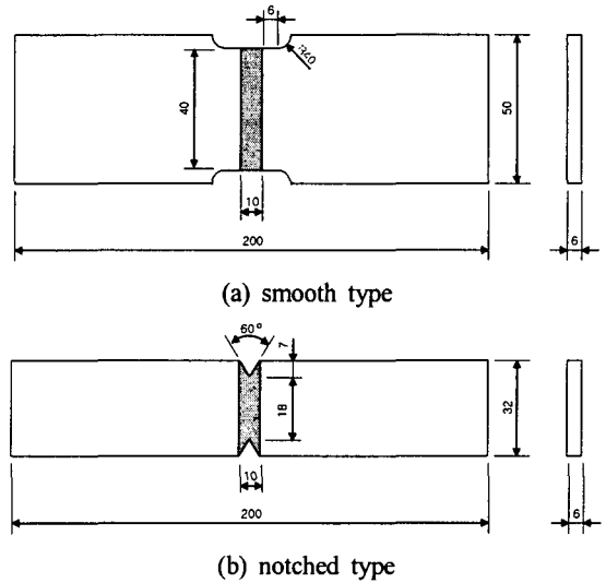
Fig. 2 Geometry of test specimen(unit:mm)
