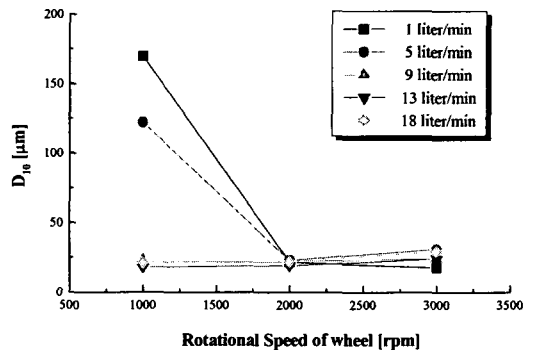
Fig. 7 Comparison of D_{10} of cutting fluid aerosol vs. rotational speed of workpiece via spin-off/splash mechanism
