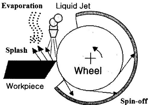
Figure 1. Aerosol generation mechanism of cutting fluid in grinding process
