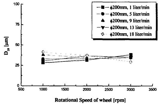
Fig. 6 Comparison of D_{10} of cutting fluid aerosol vs. rotational speed of workpiece via spin-off mechanism
