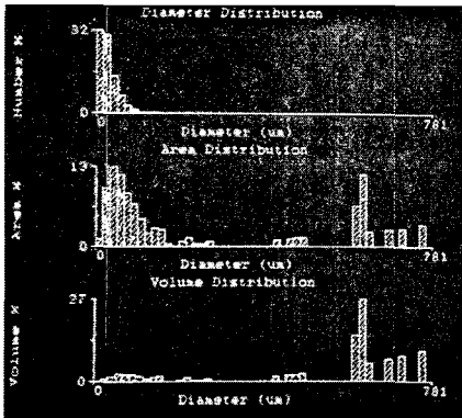
Figure 3. Comparison of cutting fluid aerosol distribution in terms of diameter, surface area, volume of cutting fluid aerosol
