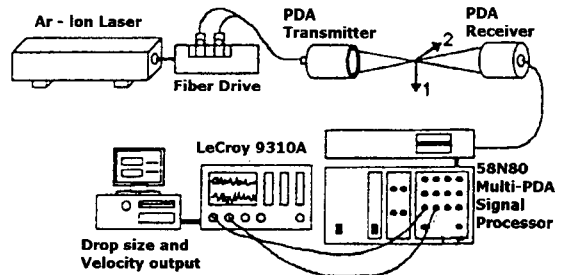
Figure 2. Dual-PDA system for cutting fluid aerosol measurement
