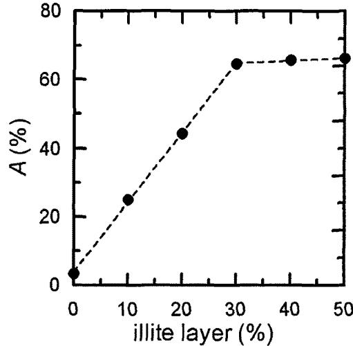
Fig. 1. Linear relationships between A and illite-layer contents.
