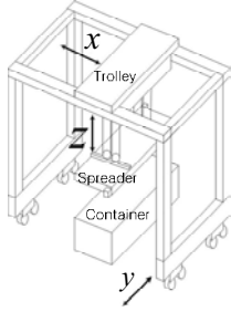
Fig. 1 Yard crane.
