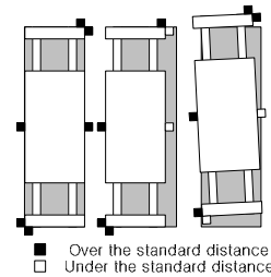
Fig. 13 Classification of the spreader arrangement state.
