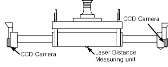
Fig. 2 Front-view of a spreader.
