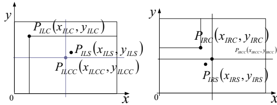
(a) left image (b) right image Fig. 6 CCD Camera image data.
