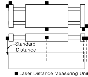
Fig. 12 Docking system with only laser distance measuring units.
