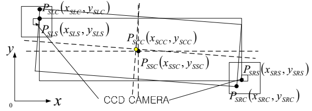
Fig. 7 Container corners and spreader corners with skew angle.
