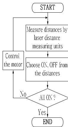
Fig. 14. Experimental flow chart using 6 laser sensors
