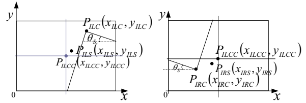
(a) Left image (b) Right image Fig. 8 CCD camera image data with skew angle.
