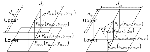
Fig. 4 Image of different height between the spreader and the container.
