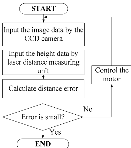
Fig. 15 Experimental flow chart using CCD cameras and laser.
