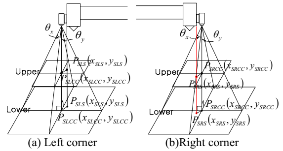
Fig. 3 Spreader corner points in the real coordinates.
