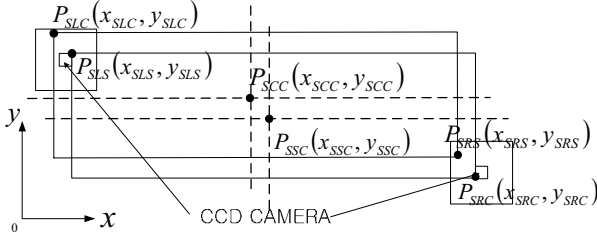
Fig. 5 Container corners and spreader corners.
