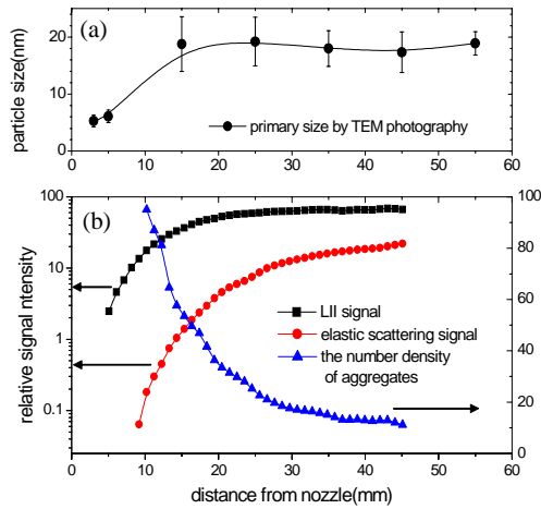
Fig. 3 The characteristics of soot evolution along the soot maximum line in ethylene IDF ( X_{C_{2H_4}}=1.0 , v_{exit}=6.9\text{cm/sec} ); (a) mean particle diameter by TEM photography (b) relative LII signal, scattering and the number density of aggregates
