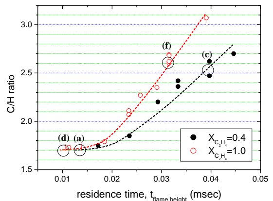
Fig. 6 The variation of C/H ratio according to residence time calculated from flame height
