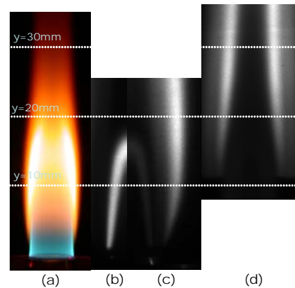
Fig. 2 OH, PAH, and soot particles distribution in ethylene IDF ( X_{\text{C}_2\text{H}_4}=1.0 , v_{\text{exit}}=6.9\text{cm}/\text{sec} , flame length:18.1mm); (a) direct photo, (b) OH signal, (c) OH signal (off line) + PAH signal, (d) scattering signal by soot particles
