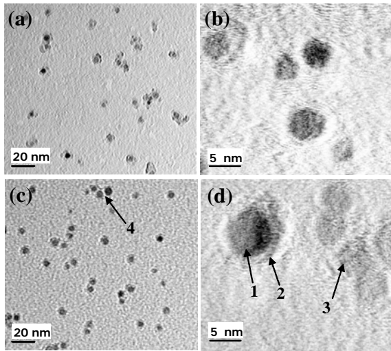
Fig. 5 TEM images of incipient and carbonaceous particles captured on carbon grid sampled from X_{C_2H_4}=1.0, 0.4 IDFs; Sampling conditions are (a),(b) y=4.0mm, H_f=28mm in X_{C_2H_4}=0.4 ; and (c), (d) y=2.5mm, H_f=18.1mm in X_{C_2H_4}=1.0
