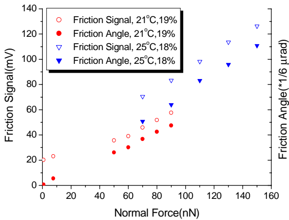
Fig. 6 The torsion angles calculated by Eq. (11) and the friction signals at each normal force.
