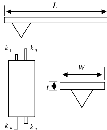
Fig. 3 Four kinds of cantilever and dimensions
