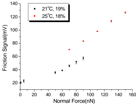
Fig. 4 The frictional signals at each normal force.
