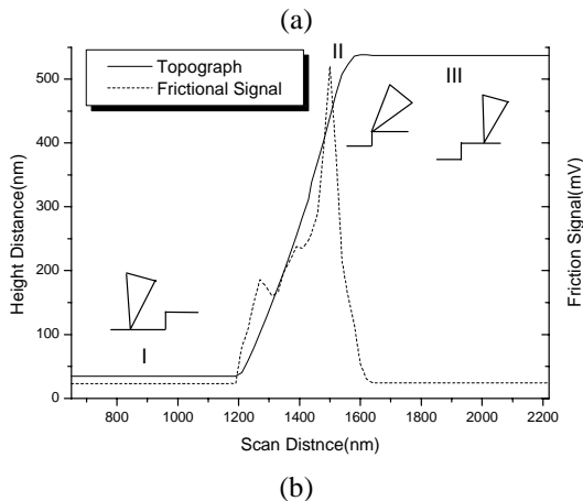
Fig. 1 (a) The location on the tip which the maximum signal happens. (b) The frictional signal and the topography at each location.
