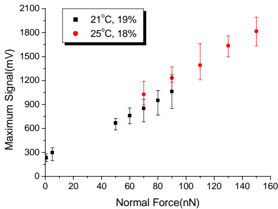
Fig. 5 The maximum signals at each normal force on the top edge of step grating.
