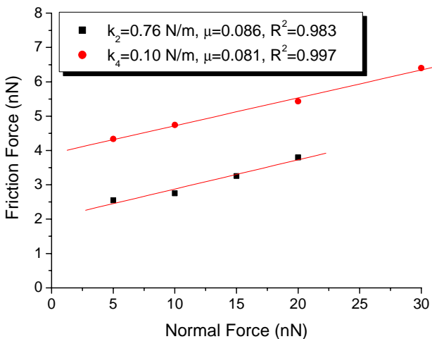
Fig. 8 The results of tests performed by cantilevers with bending stiffness of 0.76 N/m and 0.10 N/m on Mica..
