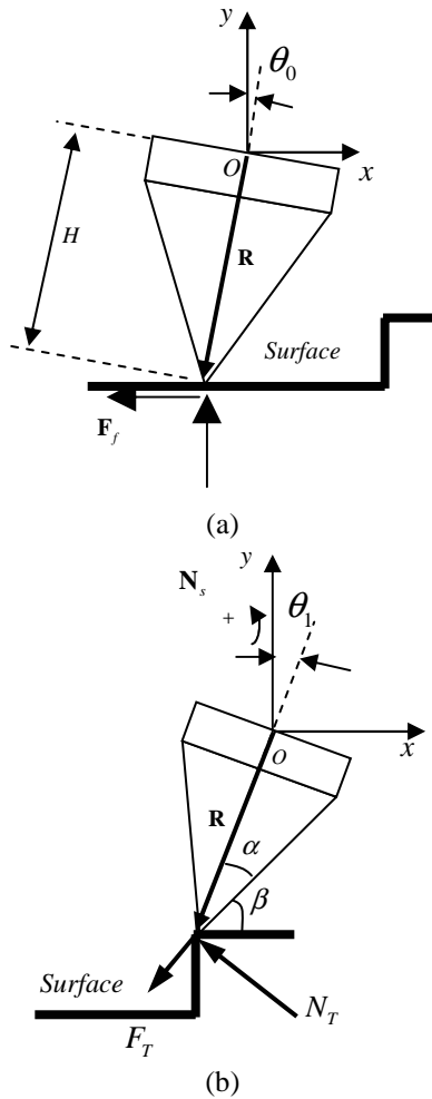
Fig. 2 The twisted shape of the tip of cantilever (a) on the flat surface and (b) on the top edge of the step grating.
