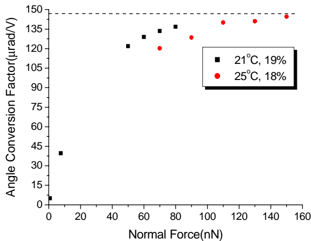
Fig. 7 The angle conversion factor at each normal force.
