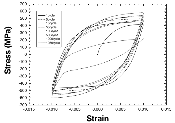
Fig. 3 Hysteresis loop of base Inconel 617 under \Delta \epsilon=0.02 low cycle fatigue
