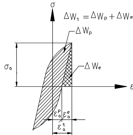
Fig. 2 Plastic and elastic strain density definition
