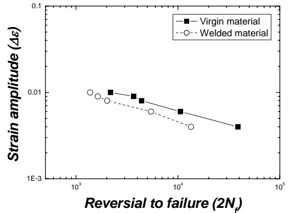
Fig. 4 Strain-life curves for low cycle fatigue test
