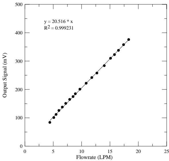
Fig. 4 Signal vs. flow rate
