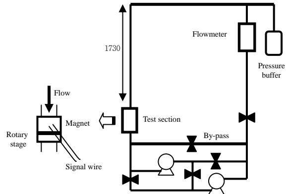
Fig. 3 Circulation loop schematic
