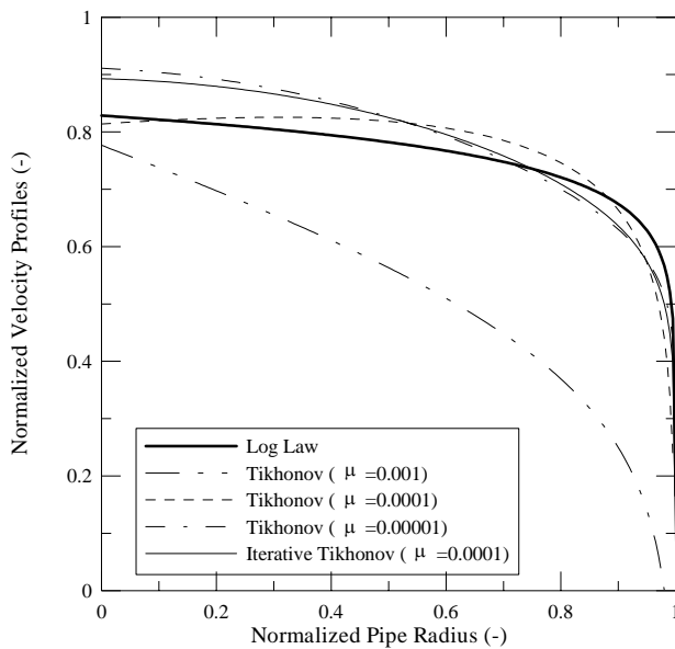
Fig. 7 Comparison between the reconstructed velocity profiles and the profile represented by log law
