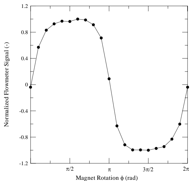
Fig. 6 Normalized flowmeter signal with respect to magnet rotation
