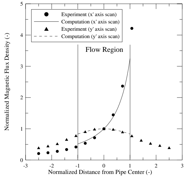
Fig. 2 Comparison between computed (Maxwell) and measured magnetic flux densities
