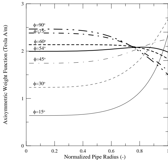
Fig. 5 Axisymmetric weight functions at various magnet rotation angles \phi
