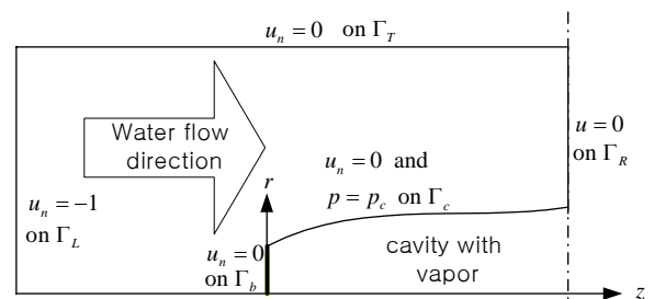
Fig. 1 Supercavitating flow problem model
