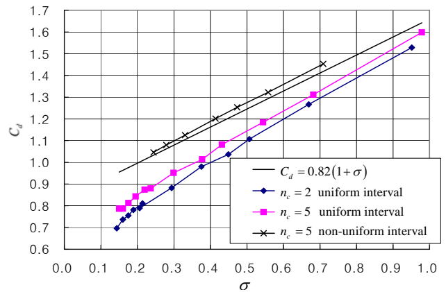
Fig. 5 Comparison between theoretical and numerical results of \sigma and C_d
