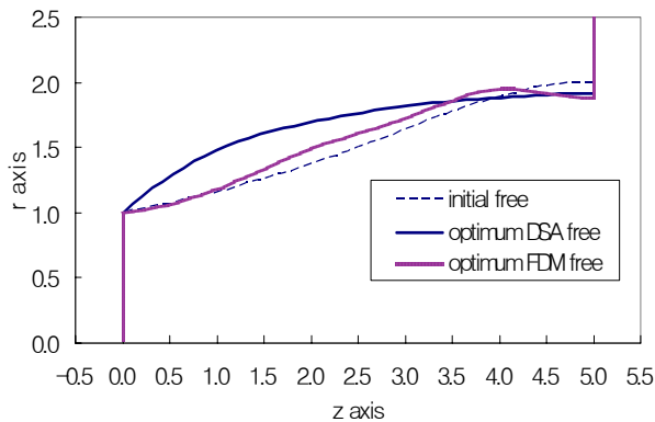
Fig. 3 Initial and optimum cavity shapes in supercavitating flow
