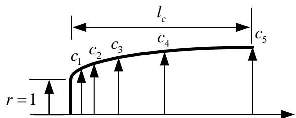
Fig. 6 Design parameters for the cavity shape with non-uniform interval
