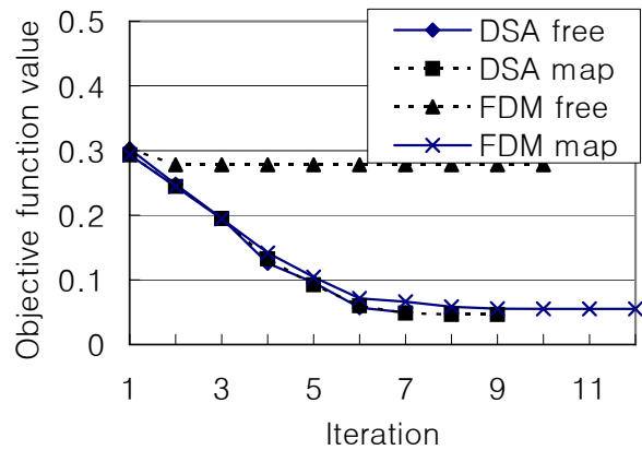
Fig. 4 Objective function history in supercavitating flow
