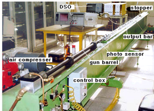
Fig. 2 General view of SHPB experimental apparatus
