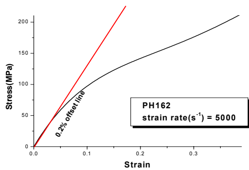
Fig. 6 Polynomial model of dynamic compressive stress-strain curve for PH162 at strain rate of 5000.
