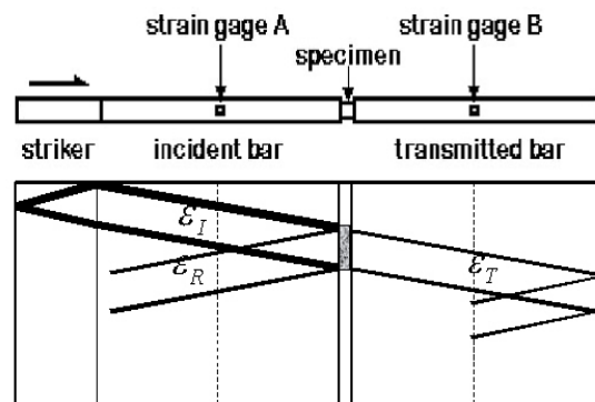
Fig. 1 A schematic diagram of specimen and elastic stress wave propagation for the compressive SHPB test
