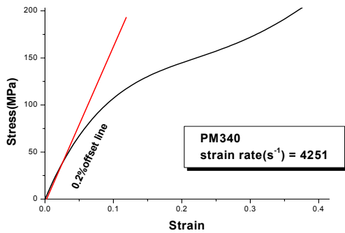
Fig. 8 Polynomial model of dynamic compressive stress-strain curve for PM340 at strain rate of 4251
