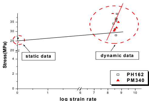
Fig. 10 Dynamic compressive yield vs. log strain rate curve for Ethylene Copolymer
