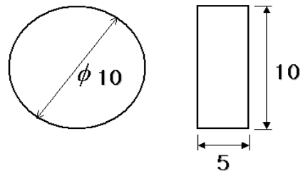
Fig. 3 Geometry of compressive specimen
