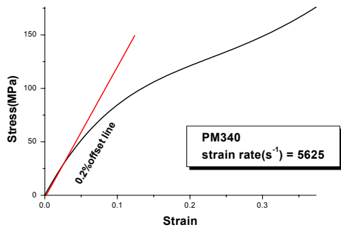
Fig. 9 Polynomial model of dynamic compressive stress-strain curve for PM340 at strain rate of 5625
