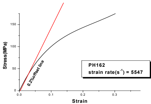
Fig. 7 Polynomial model of dynamic compressive stress-strain curve for PH162 at strain rate of 5547
