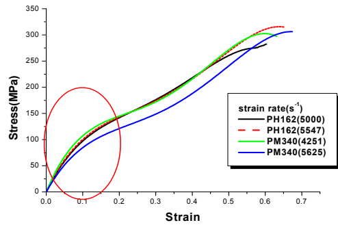
Fig. 5 Compressive stress-strain curve for Ethylene Copolymer
