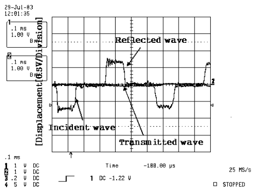
Fig. 4 Strain signal of Ethylene Copolymer recorded at oscilloscope
