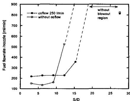
Fig 4 Effect of coflowing air on the blowout velocity of non-premixed interacting jet flame
