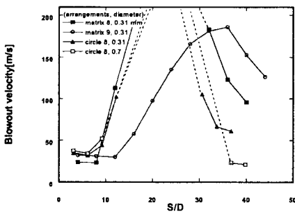
Fig. 2 Nozzle size effects on the blowout velocity of the non-premixed interacting jet flames for circular 8 nozzle.
