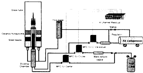
Fig. 1 Experimental apparatus
