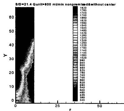
Fig. 3 Temperature distribution for s/d=21.4 and without center-nozzle
