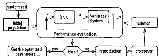
Fig.5 A functional block diagram showing the GA optimization process.
