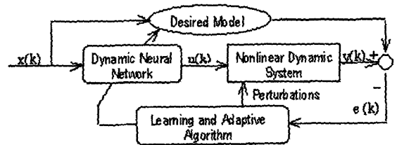
Figure 3. Control scheme for a nonlinear dynamic system using dynamic neural network
