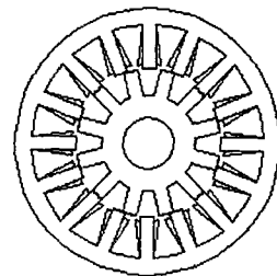
Fig.1. Cross section of the Switched Reluctance motors
