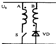
Fig.3. Main circuit of the power converter
