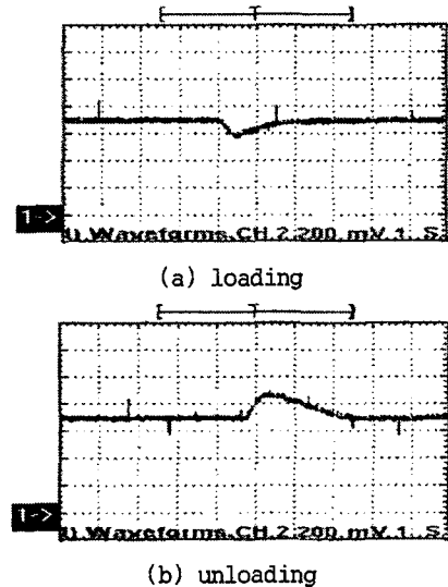
fig.5 Rotor speed curves at lacking one phase condition
