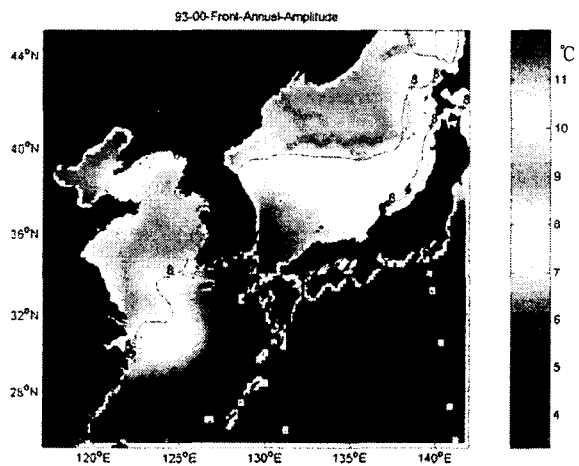
Fig. 3. Distribution of annual amplitude(°C) by harmonic analysis and Thermal Fronts (red dotted line).
