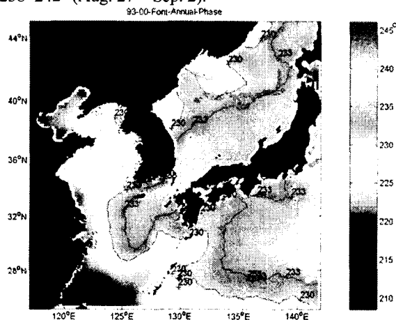
Fig. 4. Distributions of annual phase(°) by harmonic analysis and Thermal Fronts (red dotted line).
