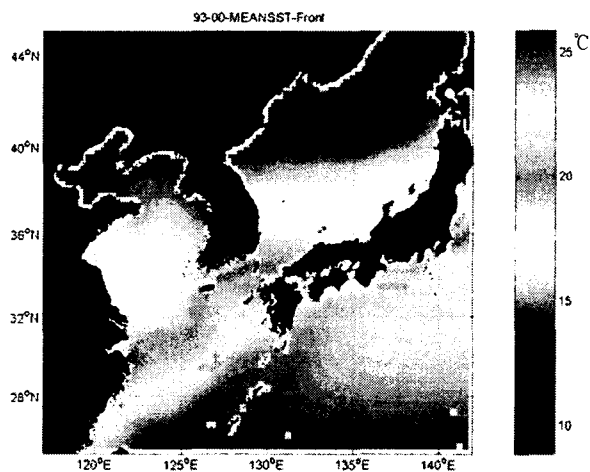
Fig. 2. Distributions of mean SST(°C) by harmonic analysis and Thermal Fronts (red dotted line).
