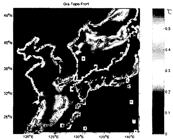
Fig. 7. Distributions of submarine topography and Thermal Fronts (red dotted line) in SST gradient image.
