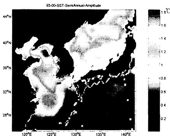
Fig. 5. Distributions of semi-annual amplitude (°C) by harmonic analysis.
