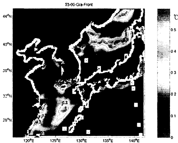
Fig. 6. Distributions of SST gradient value (°C) and Thermal Fronts (red dotted line).
