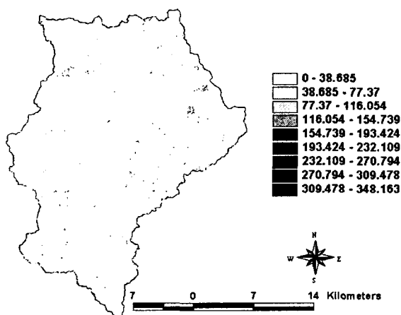
Fig. 3. Soil erosion amount distribution map
