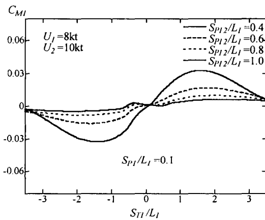
Fig. 4 Yawing moment coefficients acting on ship 1 with function of the lateral distance
