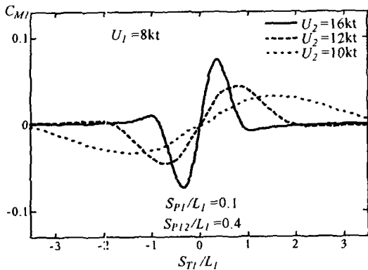
Fig. 8 Yawing moment coefficients acting on ship 1 with function of ship velocity
