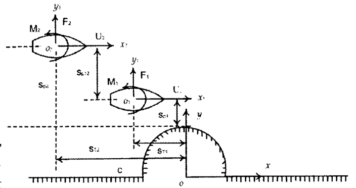
Fig. 2 Coordinate system for semi-circle bank wall
