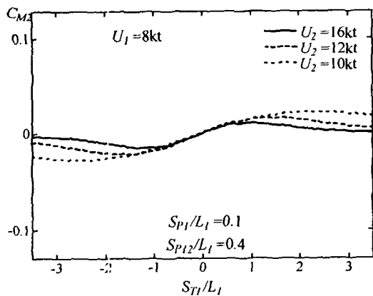
Fig. 10 Yawing moment coefficients acting on ship 2 with function of ship velocity
