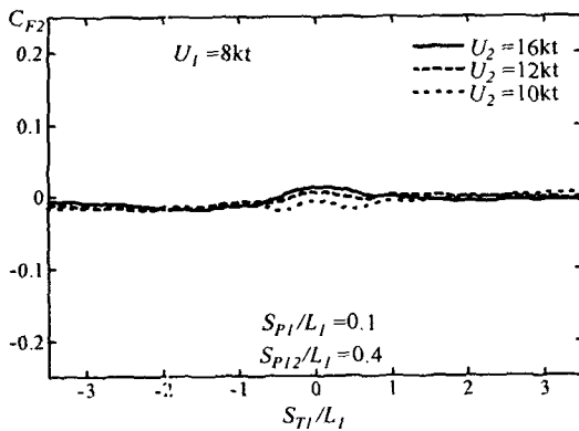
Fig. 9 Lateral force coefficients acting on ship 2 with function of ship velocity
