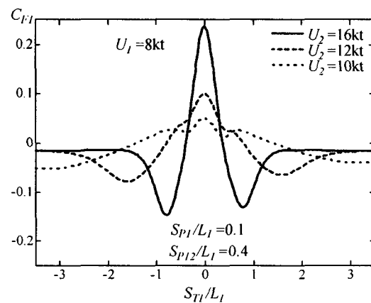
Fig. 7 Lateral force coefficients acting on ship 1 with function of ship velocity
