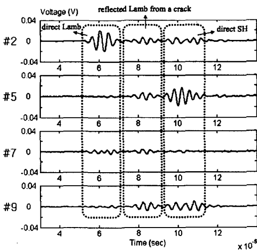
Fig. 7 The measured signals when the magnetic fluxes of the transmitting and the receiving transducers point in the direction of the crack. The transmitter and the receiver orient grid point #2, #5, #7, and #9, respectively.
