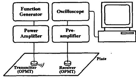
Fig. 3 The experimental arrangement (Function generator: Agilent 33120A, Power Amplifier: RAM5000, Pre-amplifier: SR560, Oscilloscope: Lecroy LT354).
