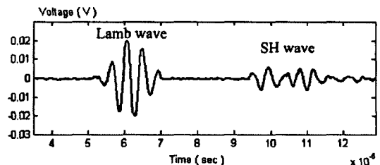
Fig. 5 The measured signal in a plate without any crack. The locations of the transducers are the same as those illustrated in Fig. 4.
