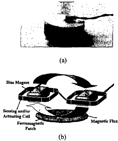
Fig. 1 (a) Manufactured OPMT (b) Schematic diagram of an OPMT
