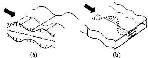
Fig. 2 Guided waves in a plate (a) Lamb wave (b) SH wave
